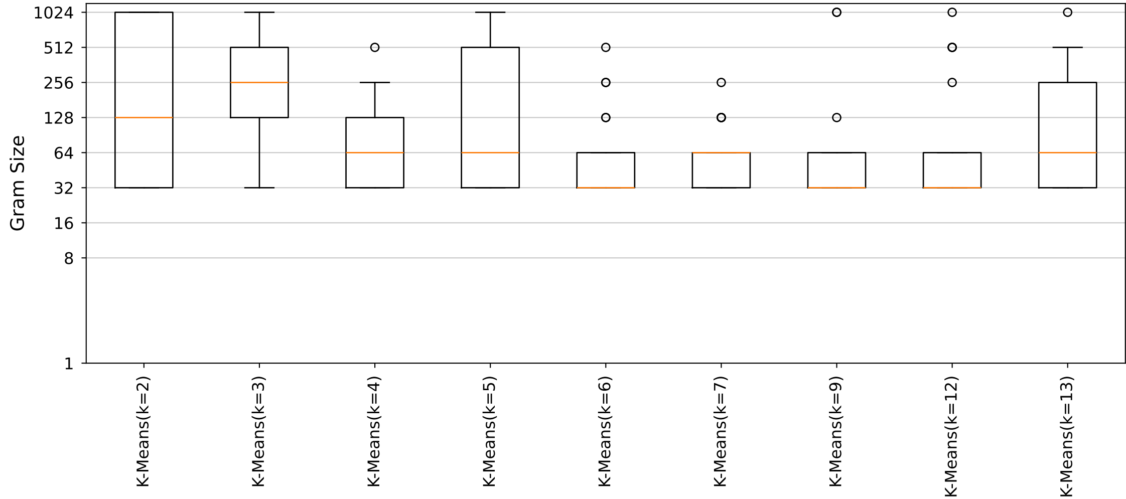
YARA Rules Gram Size Distribution (Cluster8_Size13 dataset)
